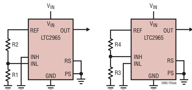
Figure 3a. Rising Edge Built-In Hysteresis
