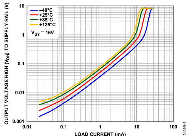
Figure 45. Output Voltage High ( V_{OH} ) to Supply Rail vs. Load Current ( I_{LOAD} ), V_{SY} = 16\text{ V}
