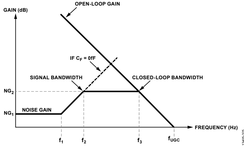
Figure 126. Transimpedance Noise Gain vs. Frequency
