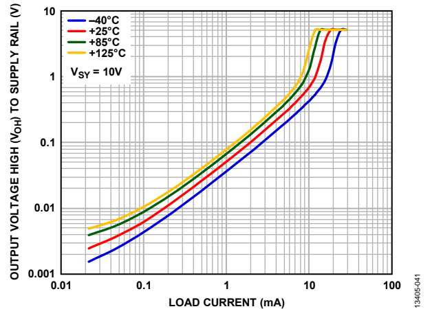
Figure 44. Output Voltage High ( V_{OH} ) to Supply Rail vs. Load Current ( I_{LOAD} ), V_{SY} = 10\text{ V}
