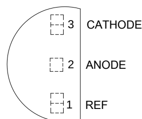
TO92 (Ammo Packing)
