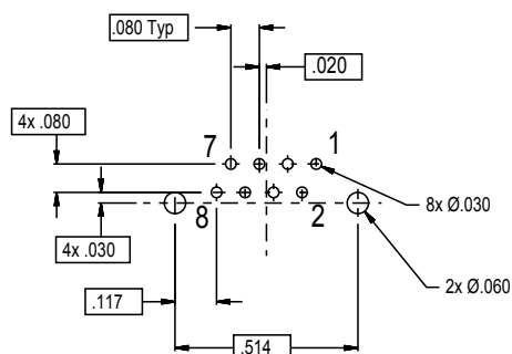
Receptacle Front View
