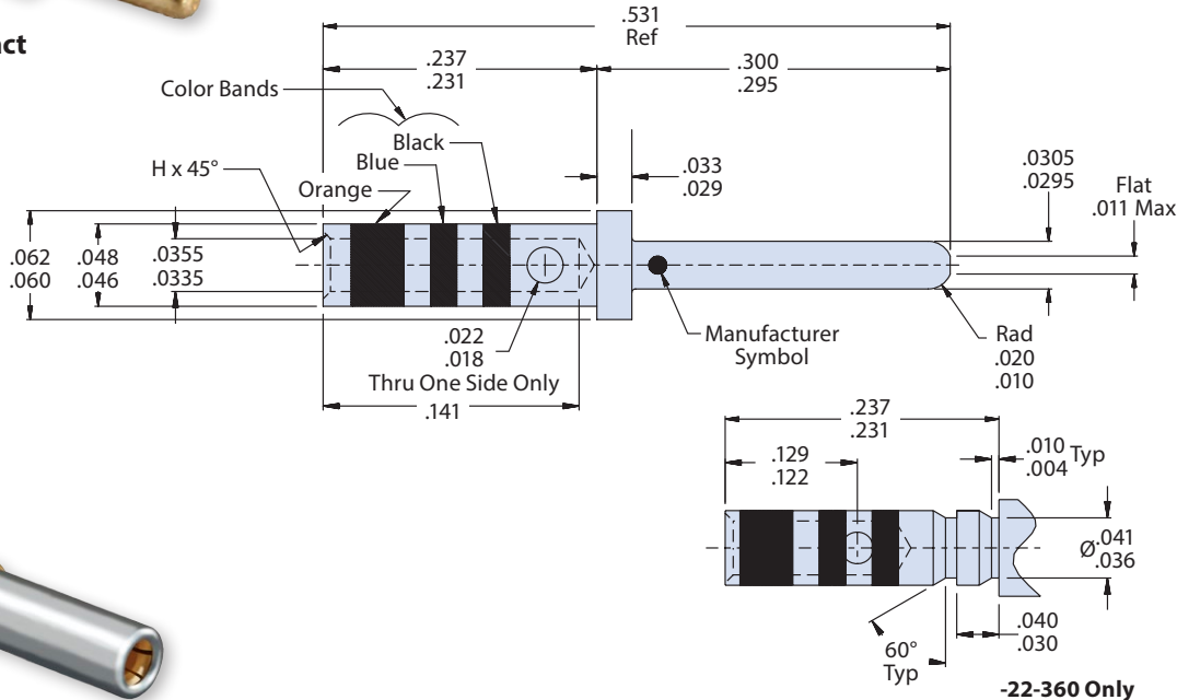
Socket Contact
