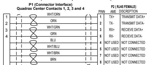
Quadrax Pin Locations
