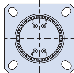
USB 2.0 Special Arrangement 4 x Size 23 Cavities (Type A)
