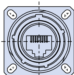
Receptacle Front View
