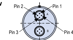
Quadrax Pin Locations
