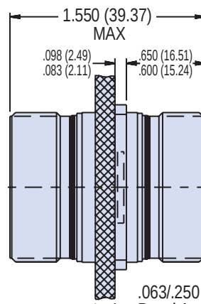
Square Flange Receptacle
