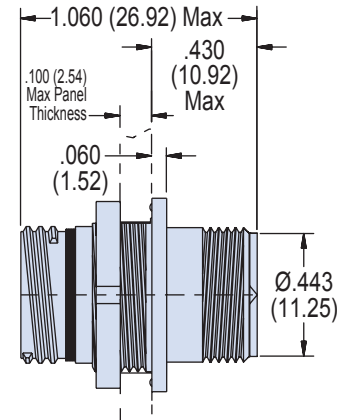
801-085-07 Jam Nut Mount Receptacle with Accessory Threads
