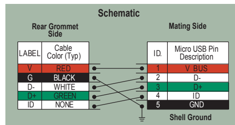
801-084-07 Jam Nut Mount Receptacle with Shield Termination Porch
