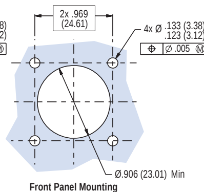
Front Panel Mounting
