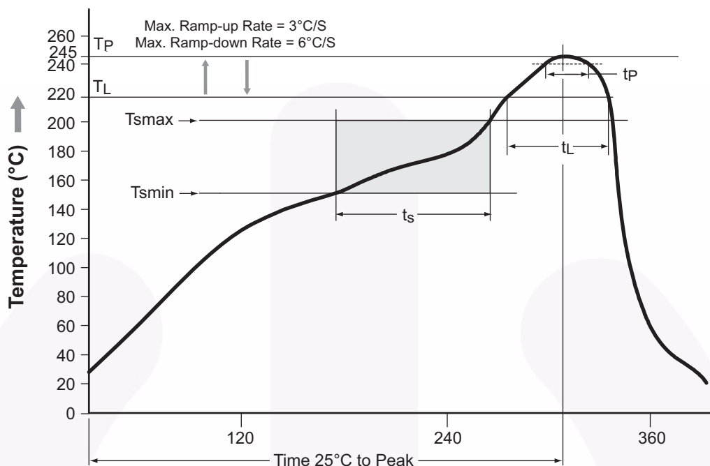
Figure 13. Reflow Profile
