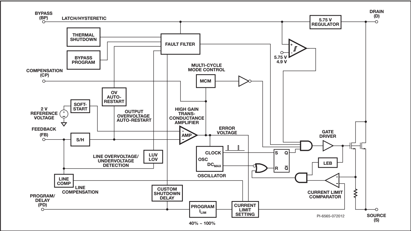
Figure 3. Block Diagram.
