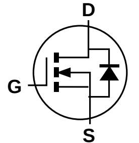
Internal Schematic
