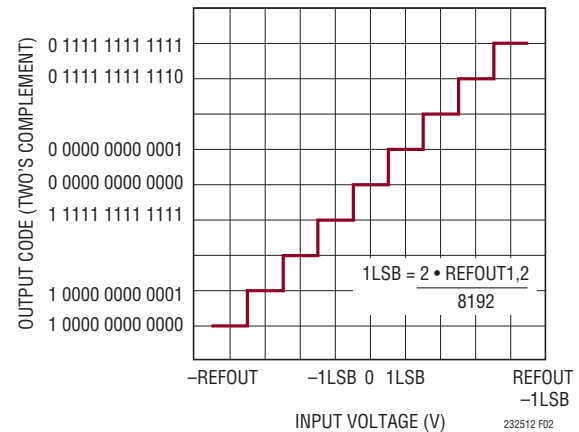
Figure 2. LTC2325-12 Transfer Function
