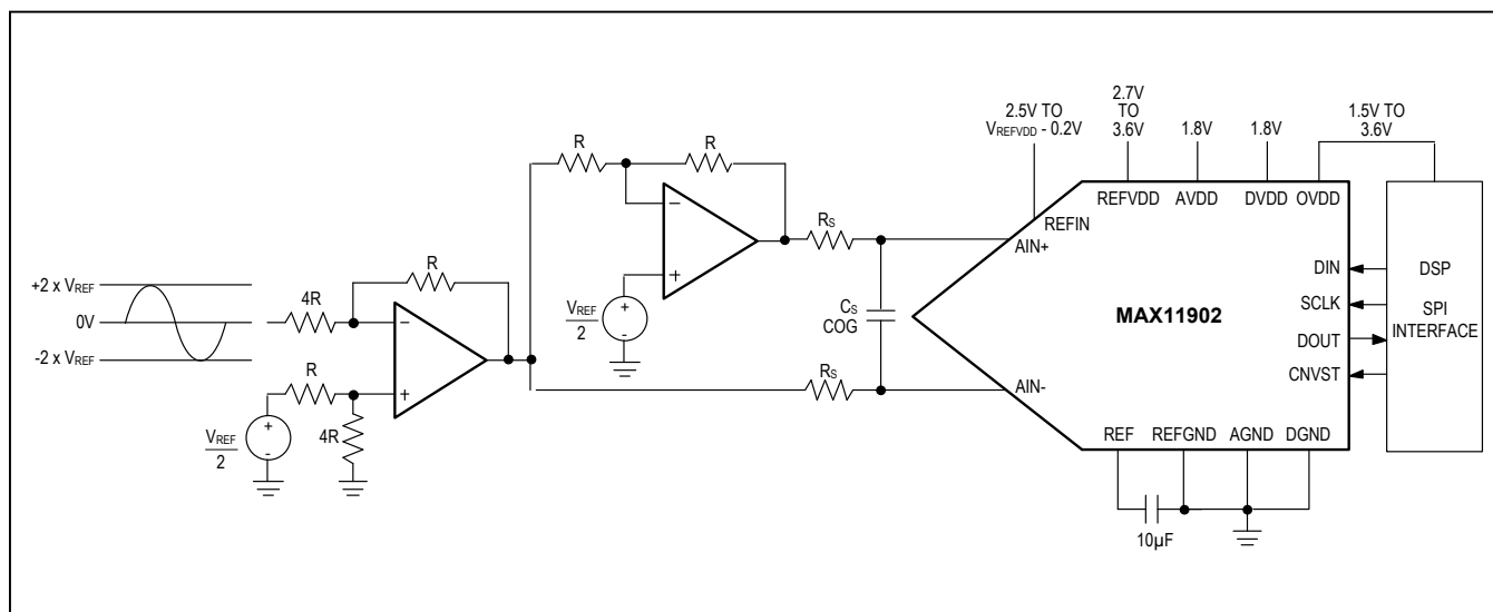
Figure 14. Bipolar Single-Ended Input
