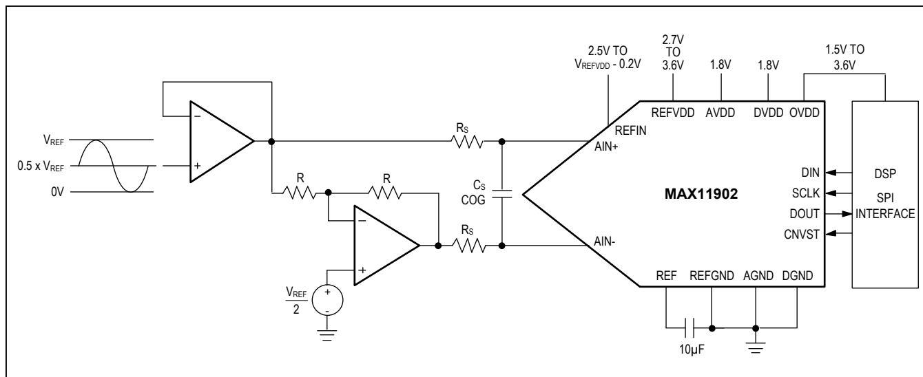
Figure 13. Unipolar Single-Ended Input
