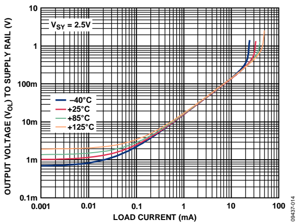
Figure 15. Output Voltage ( V_{OU} ) to Supply Rail vs. Load Current
