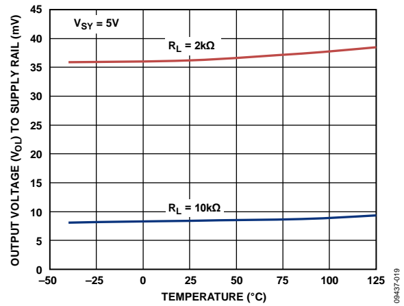
Figure 23. Output Voltage ( V_{OL} ) to Supply Rail vs. Temperature
