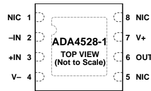
Figure 1. ADA4528-1 Pin Configuration, 8-Lead MSOP
