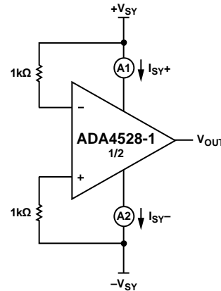
Figure 67. Comparator A
