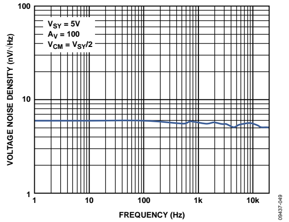
Figure 53. Voltage Noise Density vs. Frequency
