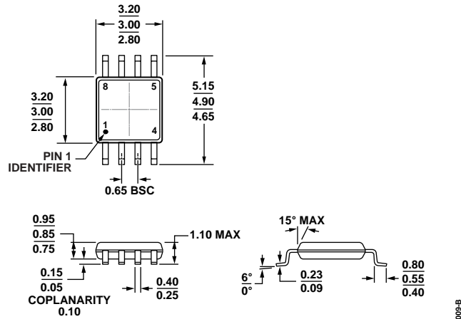
COMPLIANT TO JEDEC STANDARDS MO-187-AA Figure 71. 8-Lead Mini Small Outline Package [MSOP] (RM-8) Dimensions shown in millimeters
