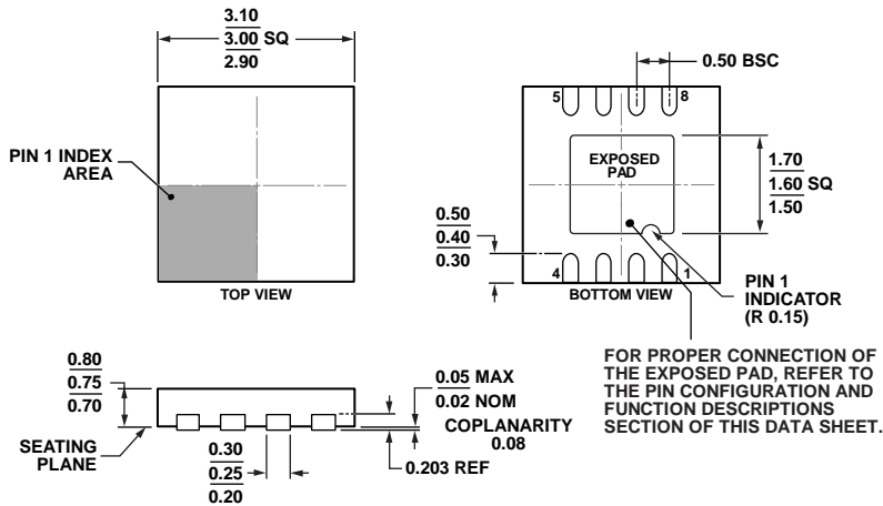
COMPLIANT TO JEDEC STANDARDS MO-229-WEED Figure 72. 8-Lead Lead Frame Chip Scale Package [LF CSP_WD] 3 mm x 3 mm Body, Very Very Thin, Dual Lead (CP-8-12) Dimensions shown in millimeters
