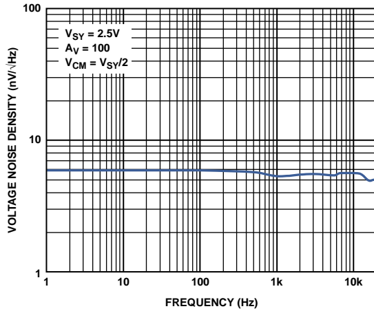
Figure 50. Voltage Noise Density vs. Frequency
