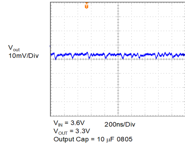
Output Ripple
