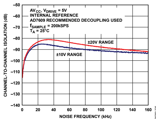
Figure 25. Channel-to-Channel Isolation
