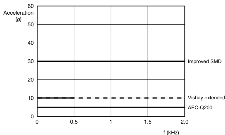
Fig. 4 - Vibration profile
