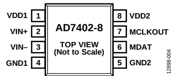
Figure 4. Pin Configuration
