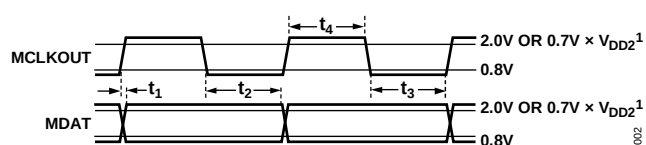
Figure 2. Data Timing
