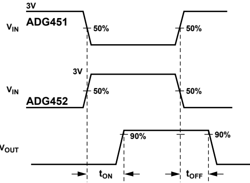
Figure 19. Switching Times
