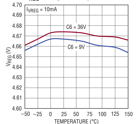
V_{\text{REG}} Voltage vs Temperature
