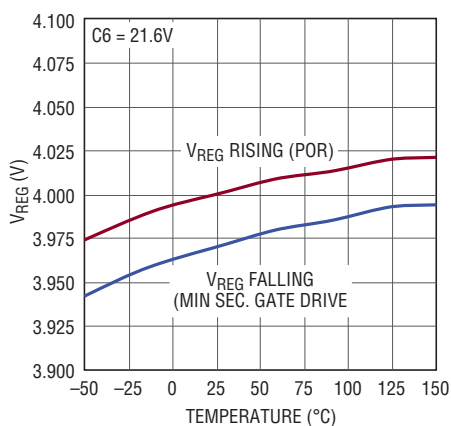
V_{\text{REG}} POR Voltage and Minimum Secondary Gate Drive vs Temperature
