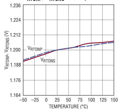
V_{\text{RTONP}} , V_{\text{RTONS}} vs Temperature
