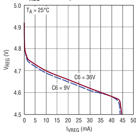
V_{\text{REG}} Load Regulation
