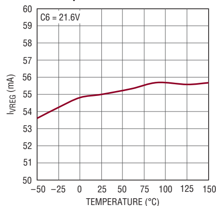
V_{\text{REG}} Short-Circuit Current Limit vs Temperature
