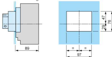
Direct Rotary Handle GV7AP03 or GV7AP04 with Conversion Accessory GV7AP05
