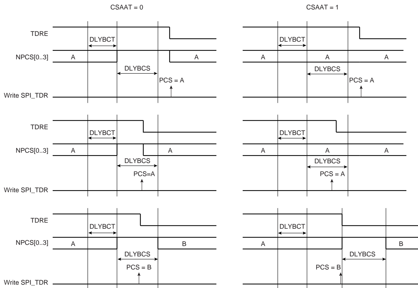
Figure 26-12. Peripheral Deselection
