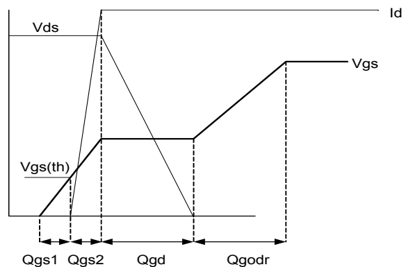
Fig 18b. Gate Charge Waveform
