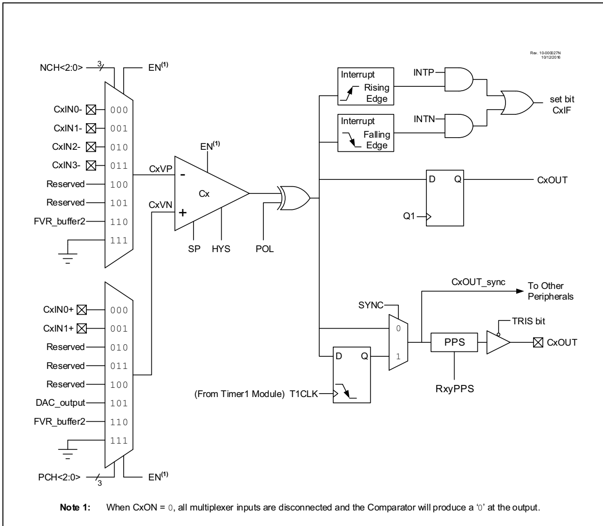
FIGURE 38-2: COMPARATOR MODULE SIMPLIFIED BLOCK DIAGRAM
