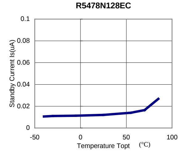
20) Standby Current vs. Temperature Vdd=3.9V, V-=0V
