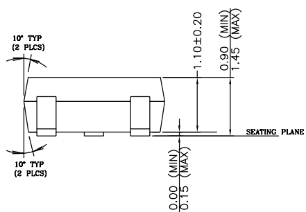
SIDE VIEW 1
