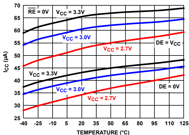
FIGURE 13. ISL32600E, ISL32601E STATIC SUPPLY CURRENT vs TEMPERATURE
