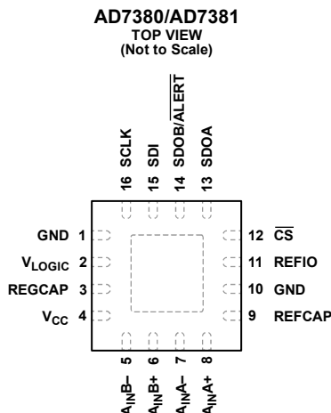
Figure 8. Pin Configuration
