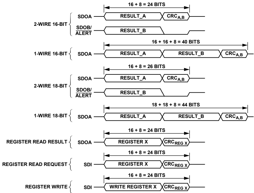
Figure 43. CRC Operation
