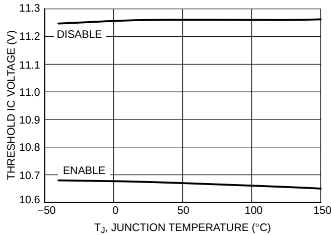
Figure 11. NCV887720 Threshold IC Voltage vs. Temperature
