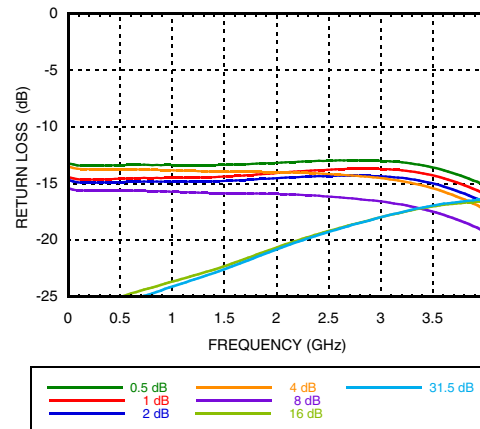
Return Loss RF1, RF2 (Only Major States are Shown)
