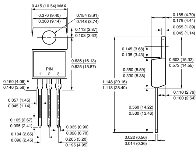
TO-220AB
