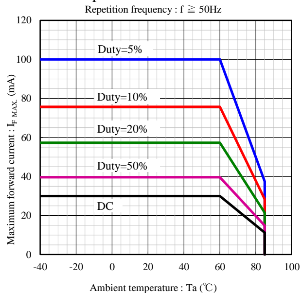
Ambient temp. vs. Maximum forward current
