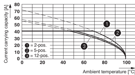
Derating curve for: IPC 5/...-ST-7,62 with IPC 5/...-G-7,62 Conductor cross section = 10 mm²
