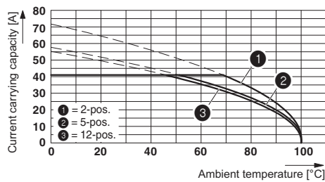
Derating curve for: IPC 5/...-ST-7,62 with PC 5/...-ST-7,62 Conductor cross section = 10 mm²
