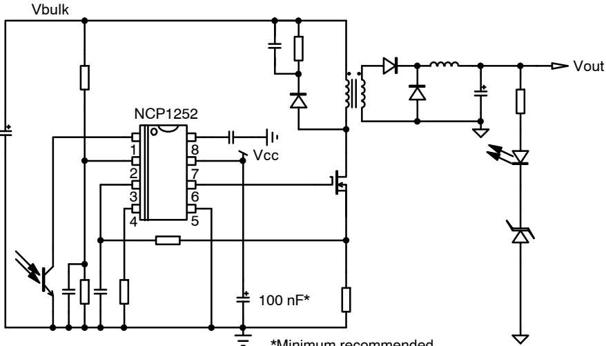
Figure 1. Typical Application
