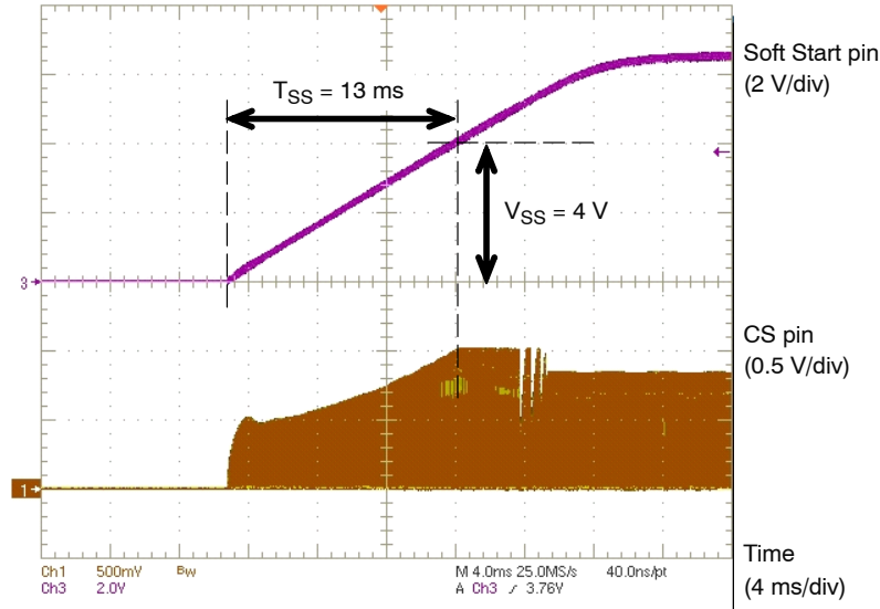
Figure 33. Soft Start Example
