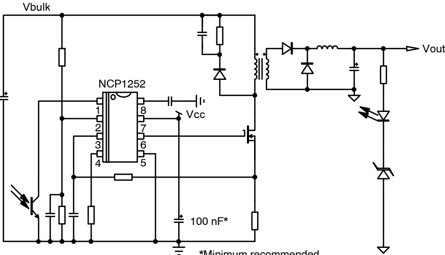
Figure 1. Typical Application
