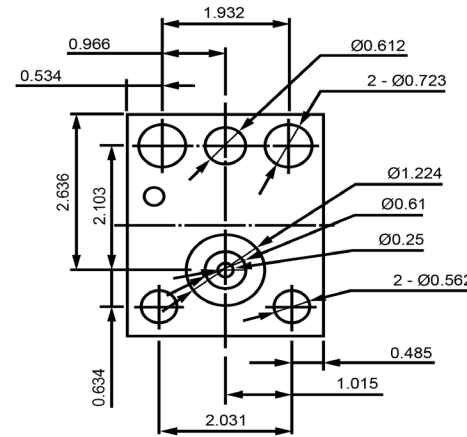
BOTTOM VIEW (1)
