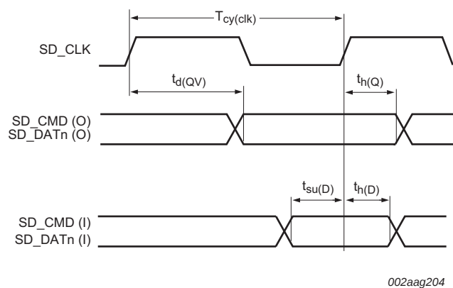
Fig 39. SD/MMC timing
