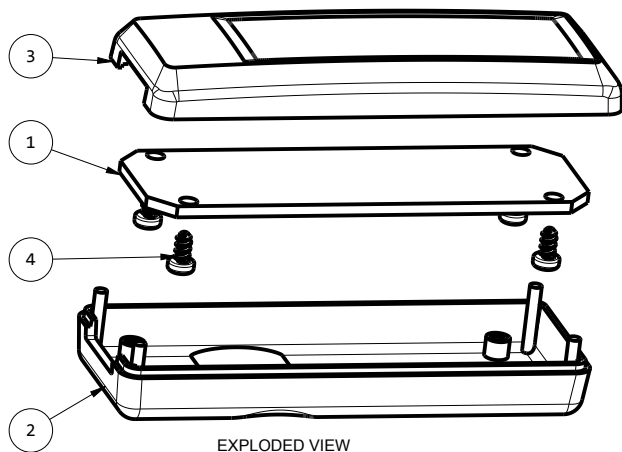
EXPLODED VIEW SCALE 1.000
