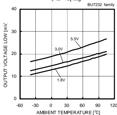
Fig. 74 Output Voltage Low - Ambient Temperature (RL=10[kΩ])
