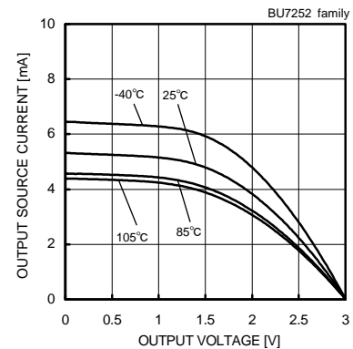
Fig. 31 Output Source Current - Output Voltage(VDD=3[V])
