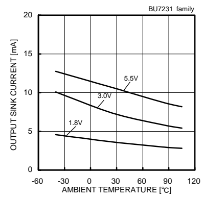
Fig. 56 Output Sink Current - Ambient Temperature ( V_{OUT}=V_{SS}+0.4[V] )
