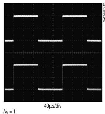
LARGE-SIGNAL TRANSIENT RESPONSE (NONINVERTING)
