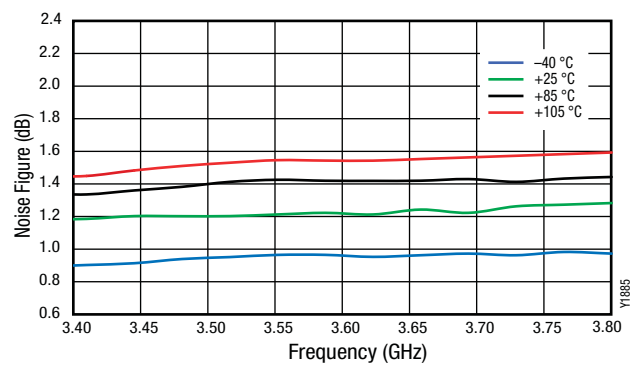
Figure 25. Noise Figure vs Frequency
