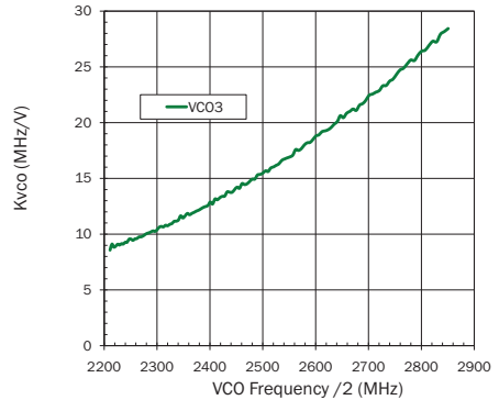
VCO3 Frequency versus Kvco LO Divide by 2
